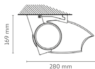
Ceiling installation
