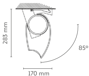
85° Ceiling installation
