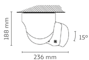
15° Ceiling installation
