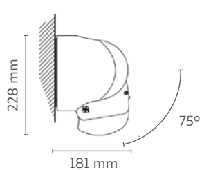
75° Wall installation
