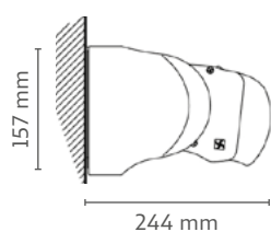
Wall installation
