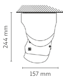
90° Ceiling installation
