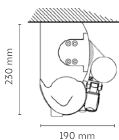
Ceiling installation
