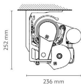
Ceiling installation
